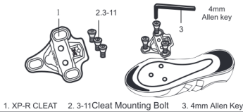
1. XP-R CLEAT 2. 3-11 Cleat Mounting Bolt 3. 4mm Allen Key
